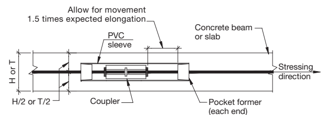
Fig. 6 – Coupler Installation Details
