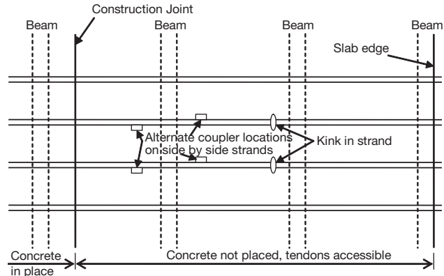
Fig. 4 – Replacing Damaged Tendons
