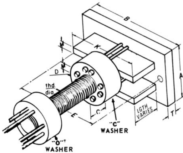
Fig. 13 – Sample Intermediate Anchorage Assembly for Unbonded Button-Headed Wire Tendons 7
