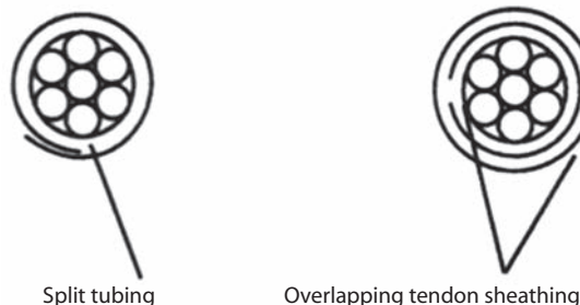
Fig. 7 – Procedure for Sheathing Repair
