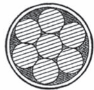
Fig. 2 – Plastic Sheathing Techniques for Unbonded Single Strand Tendons 3
