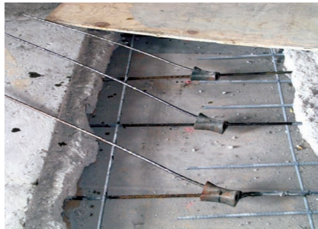
Fig. 10 – Intermediate Stressing Anchors for Slab Repair
