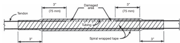
Fig. 8 – Restored Sheathing on a Damaged Tendon
