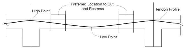
Fig. 3 – Preferred Location to Cut and Repair Tendons
